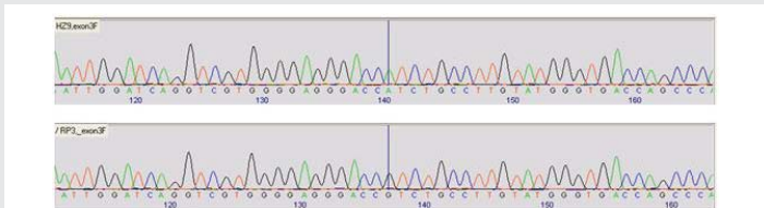
Figure 6: Staden chromatogram traces of missense mutation c.1103G>A (p.R368H) in a homozygous state. The top trace shows the mutant sequence and the bottom trace is the reference wildtype sequence. Found in patient HZ9.
