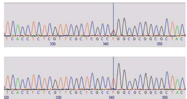
Figure 4: Staden chromatogram traces of missense mutation c.230T>C (p.L77P) in TC7. The top trace shows the mutant sequence and the bottom trace is the reference wild type sequence.
